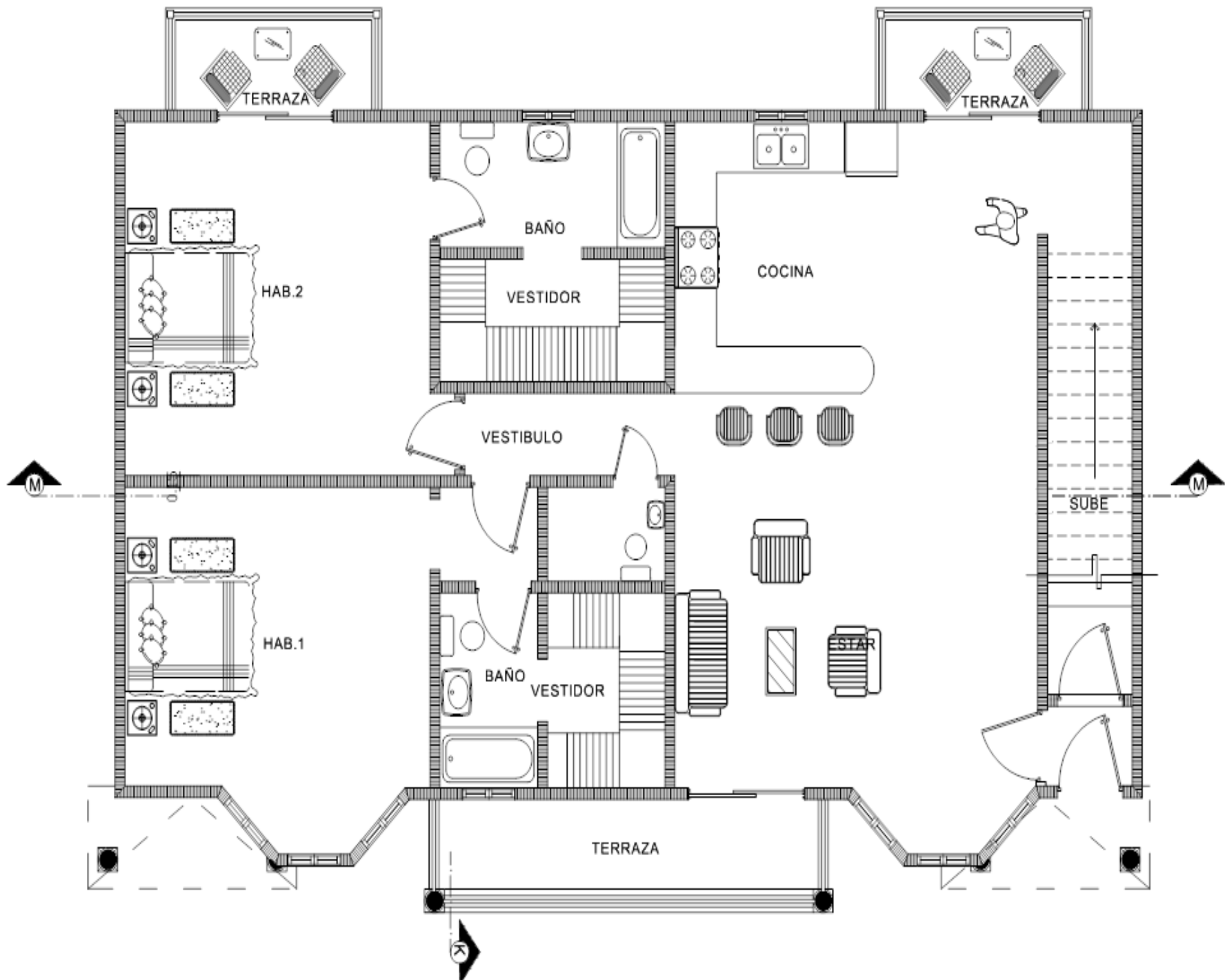
Building A Unit 1
